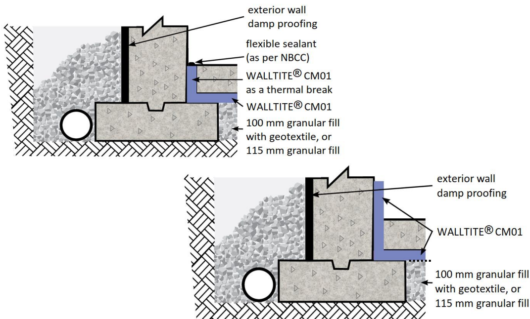
Figure 1. Application of “WALLTITE® CM01” for radon control beneath concrete slab, with geotextile/100 mm gravel or without geotextile/115 mm gravel bed.
