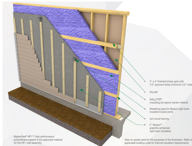
Figure 1. Illustration of BASF HP+ Wall XR Series
