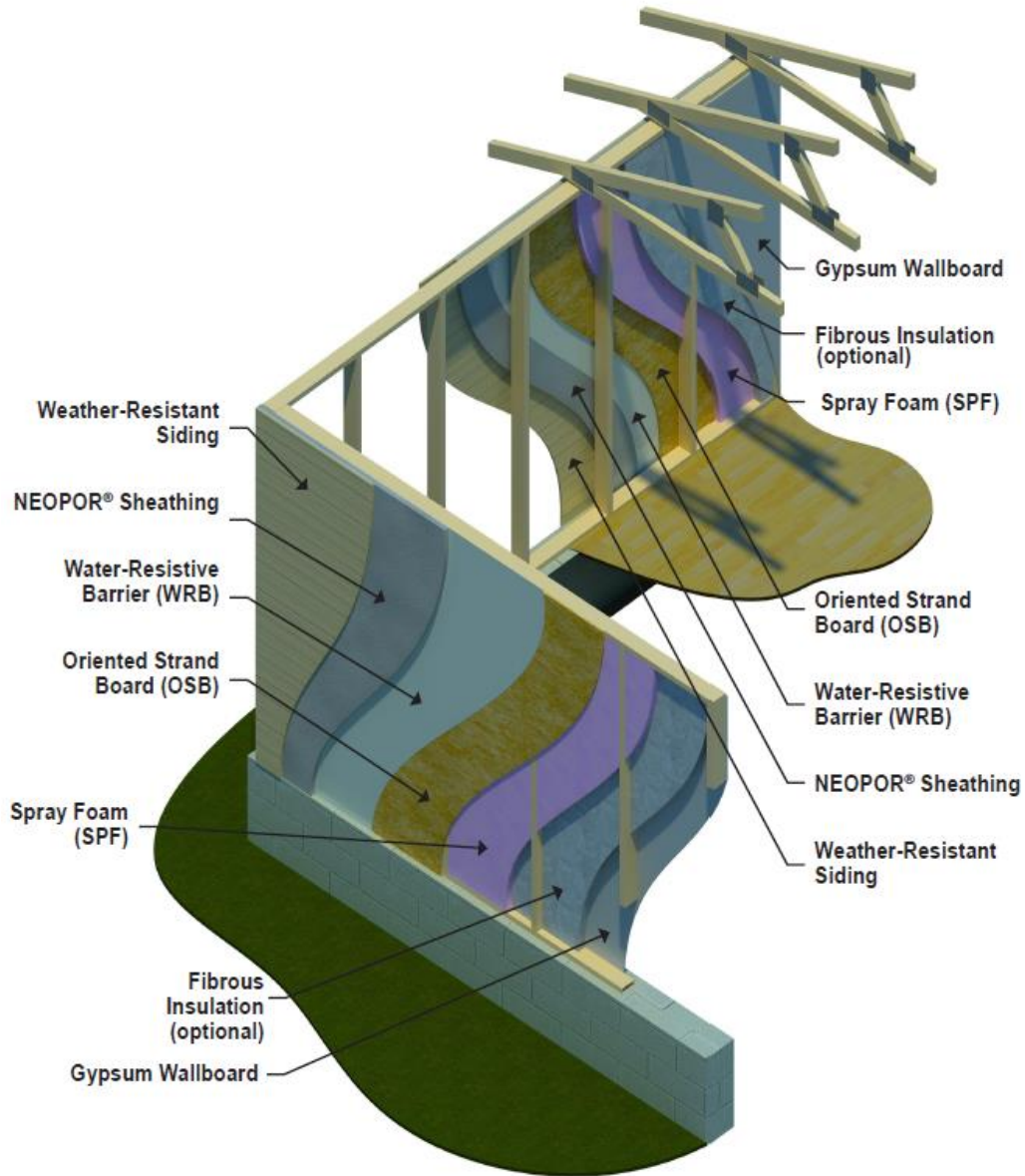
Figure 1a: Illustration of BASF HP+ Wall X Series
