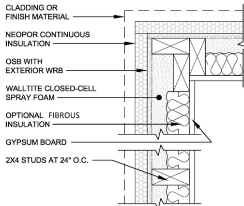
Figure 1b: Cross Section of BASF HP+ Wall X Series Layers
